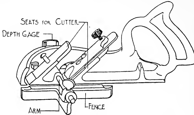
FIG. 68. RABBET AND FILLETSTER PLANE.
